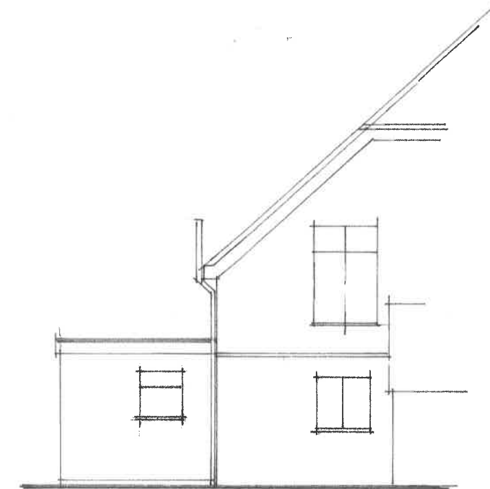
SIDE ELEVATION PROPOSED NE 1-100
