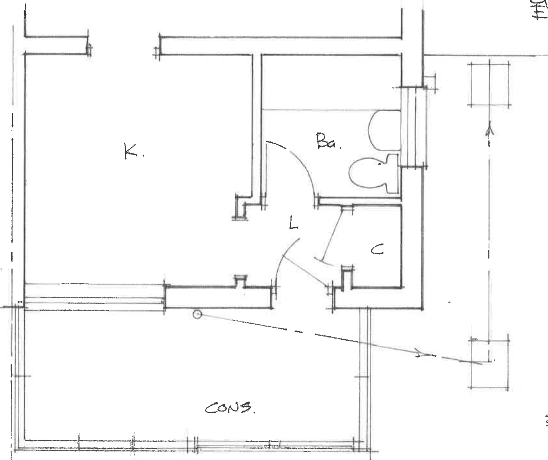
GROUND FLOOR PLAN EXISTING. 1-50.
