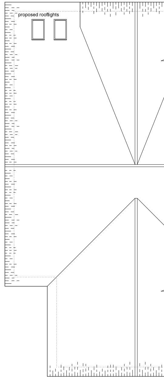
Roof Plan
