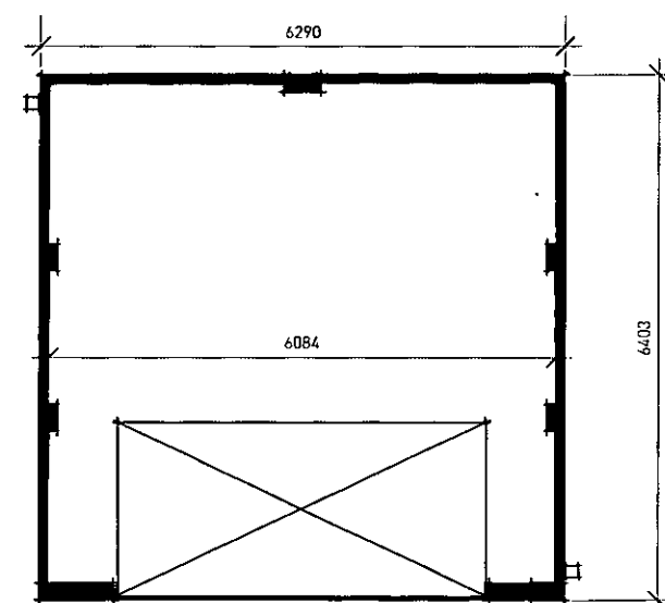
PLAN - DOUBLE
