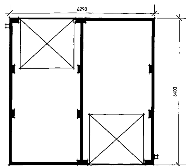
PLAN - TWIN
