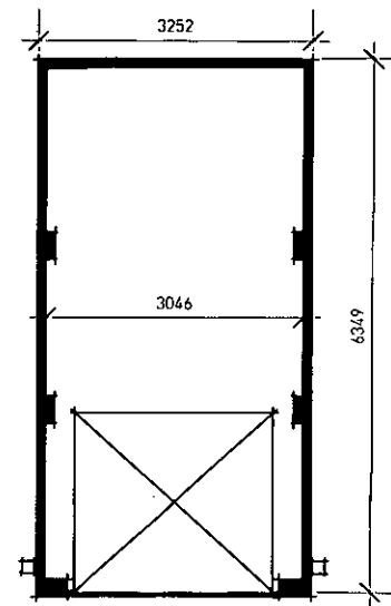
PLAN - SINGLE
