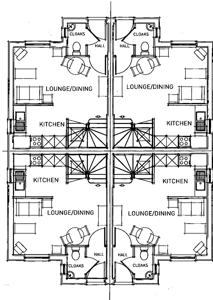
GROUND FLOOR
