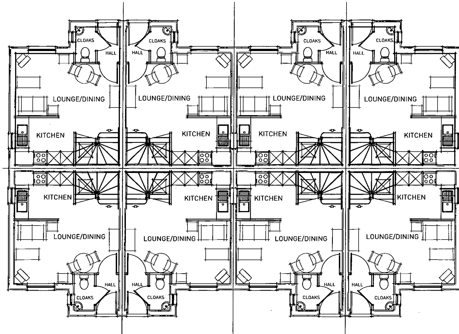
GROUND FLOOR
