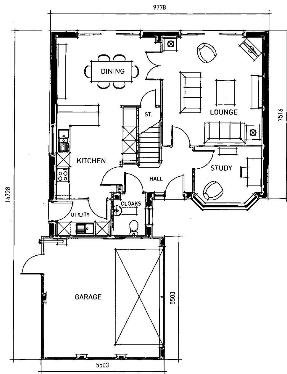
GROUND FLOOR
