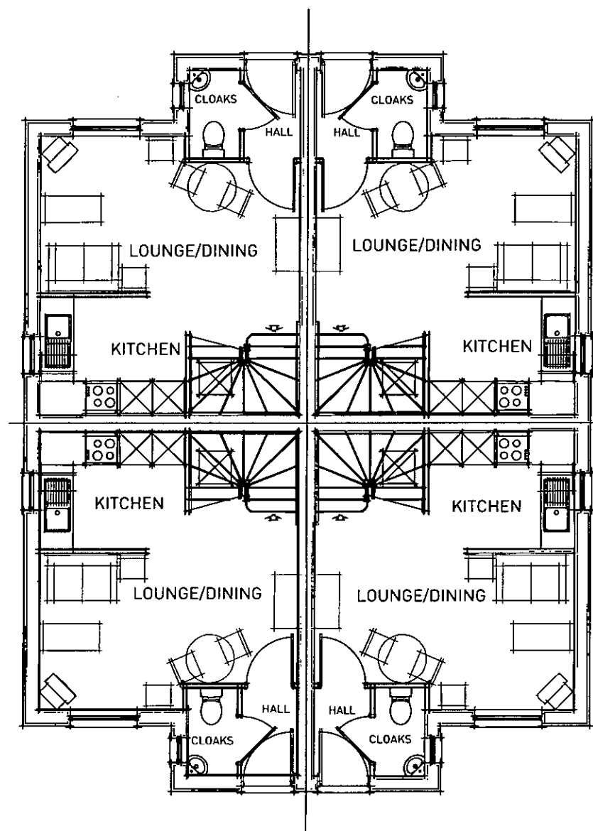
GROUND FLOOR
