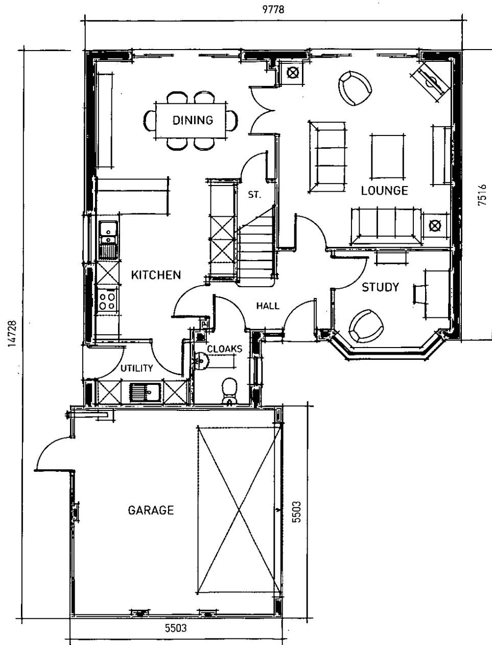
GROUND FLOOR
