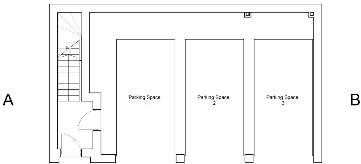
Ground Floor Plan 1:100
