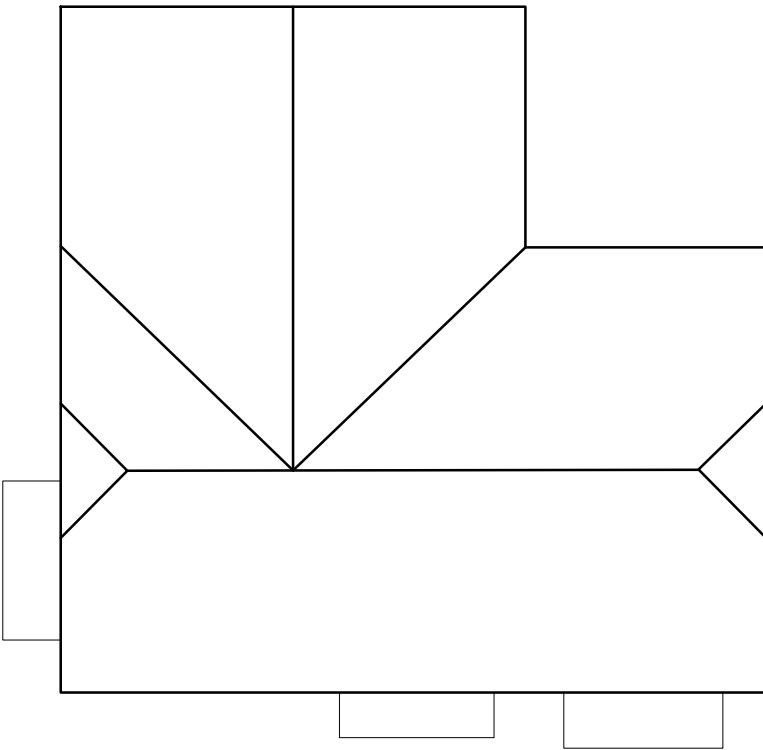
Roof Plan 1:100
