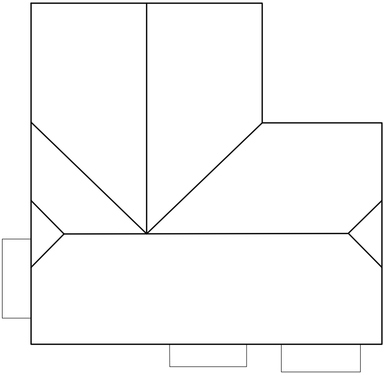
Roof Plan 1:100
