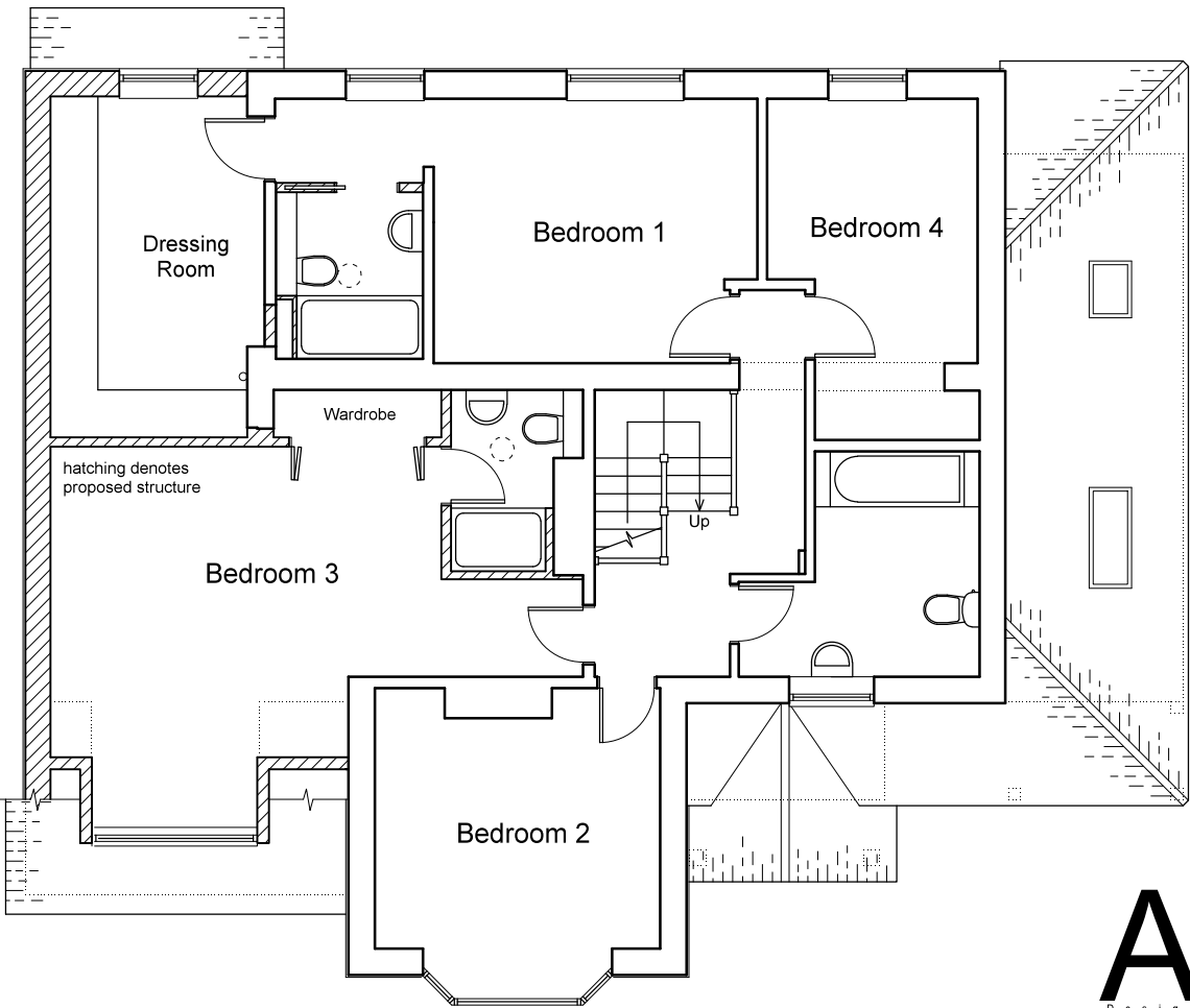
First Floor Plan Option Five
