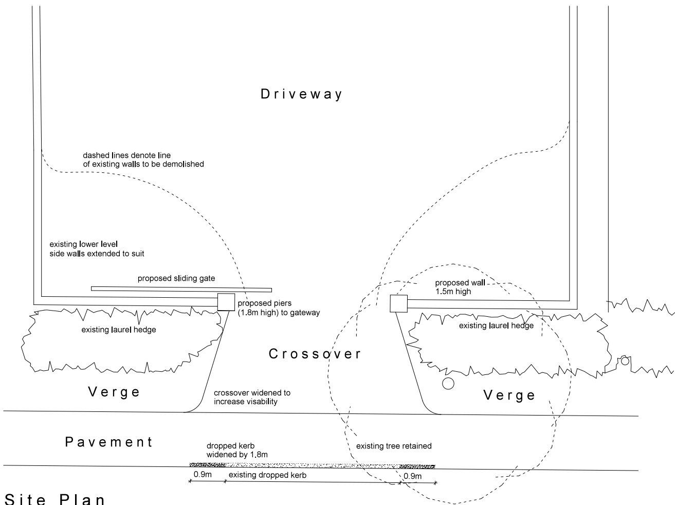
Site Plan
