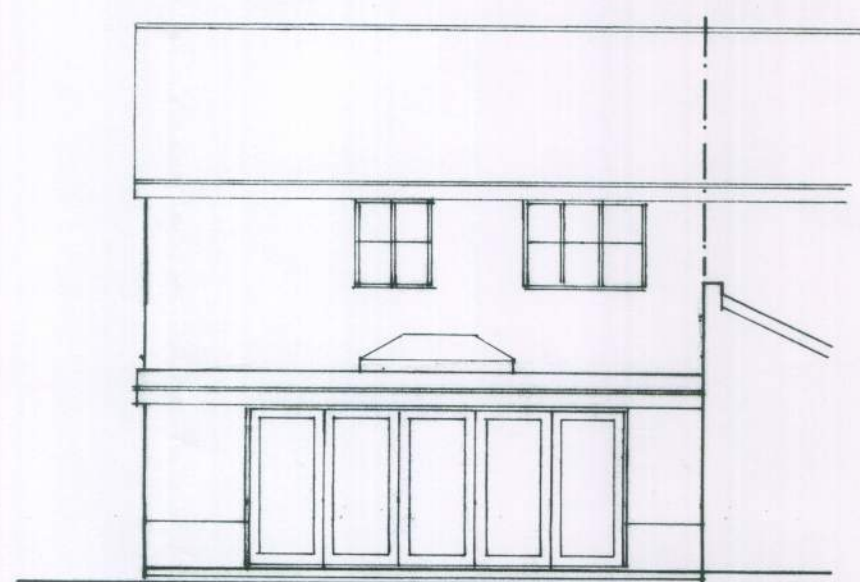
rear 1:100
