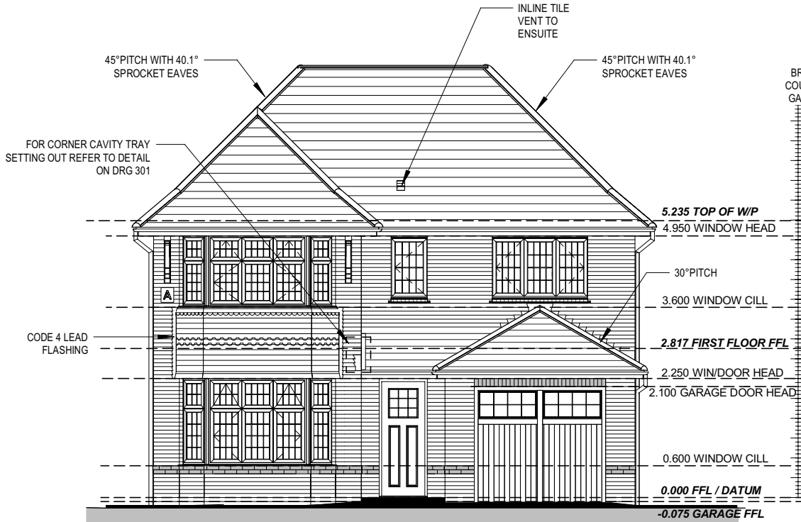
FRONT ELEVATION
