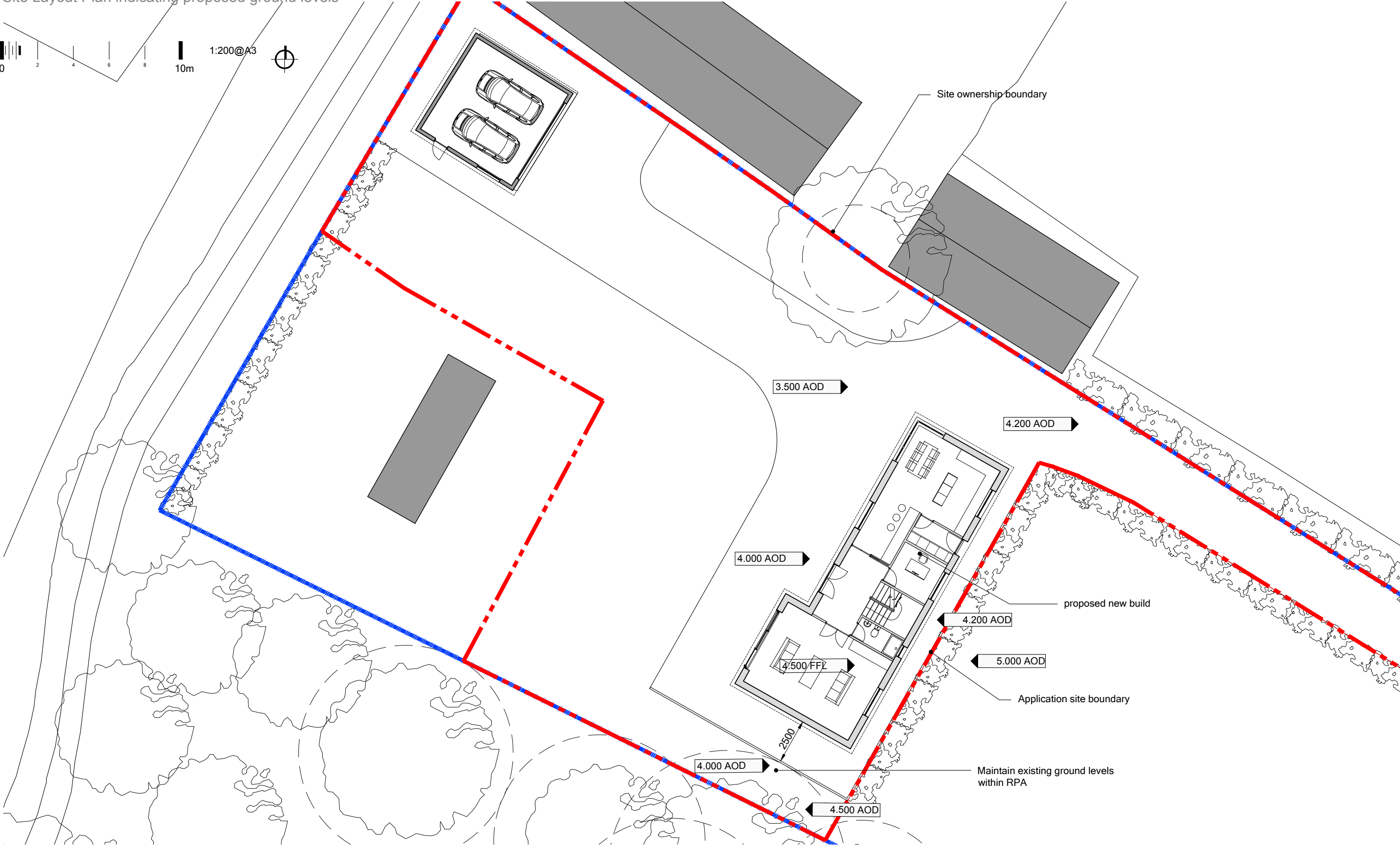
Site Layout Plan indicating proposed ground levels
