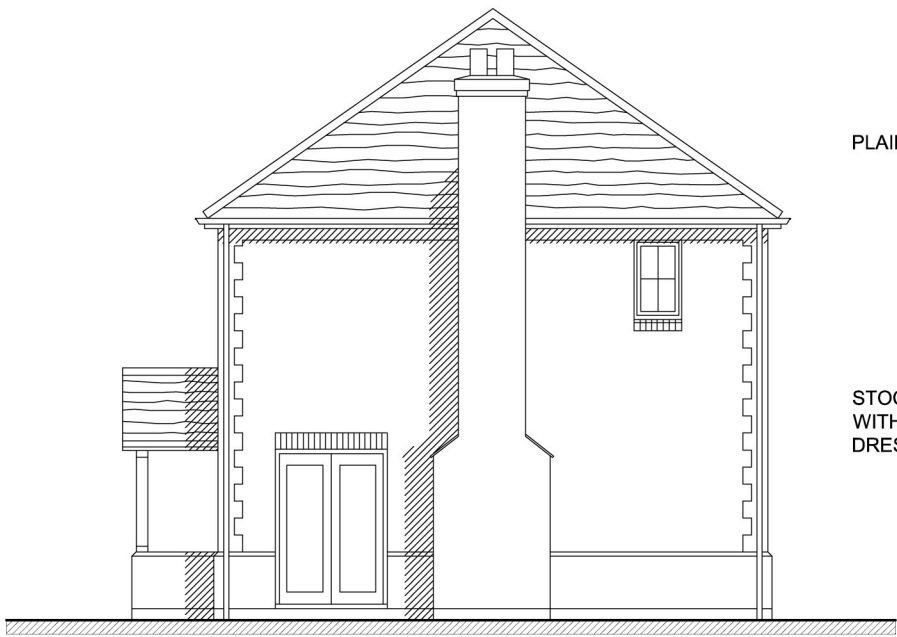
Plot 5 East Elevation
