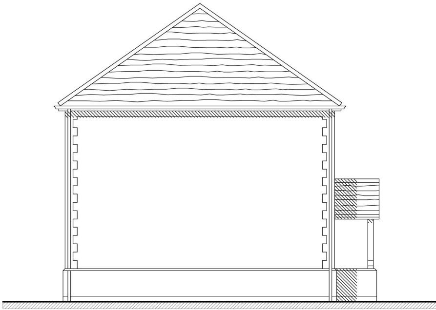
Plot 5 West Elevation
