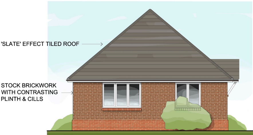
East Elevation
