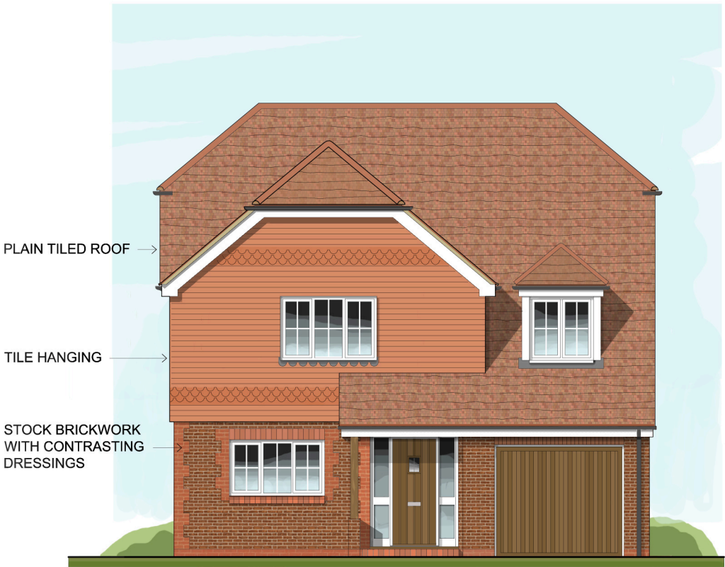
East Elevation
