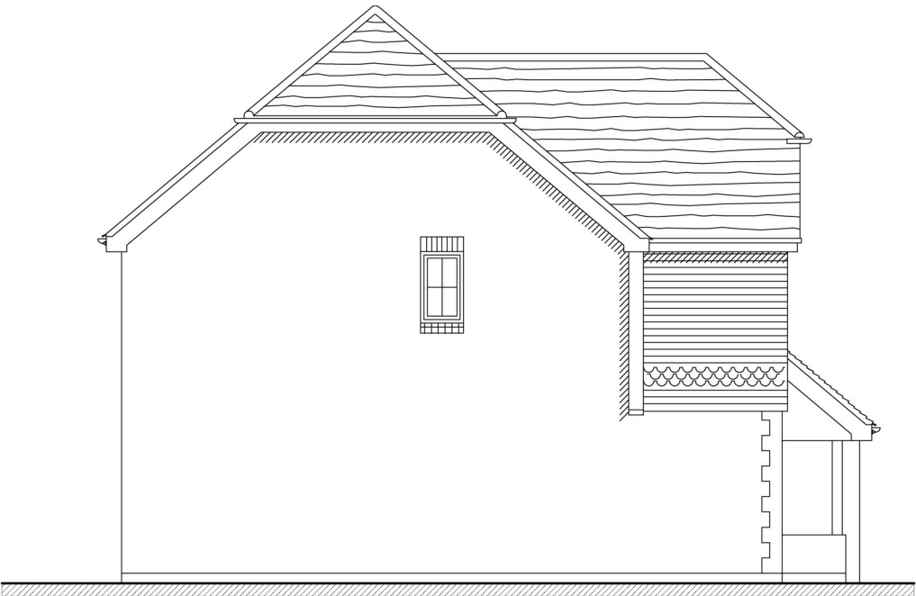
South Elevation
