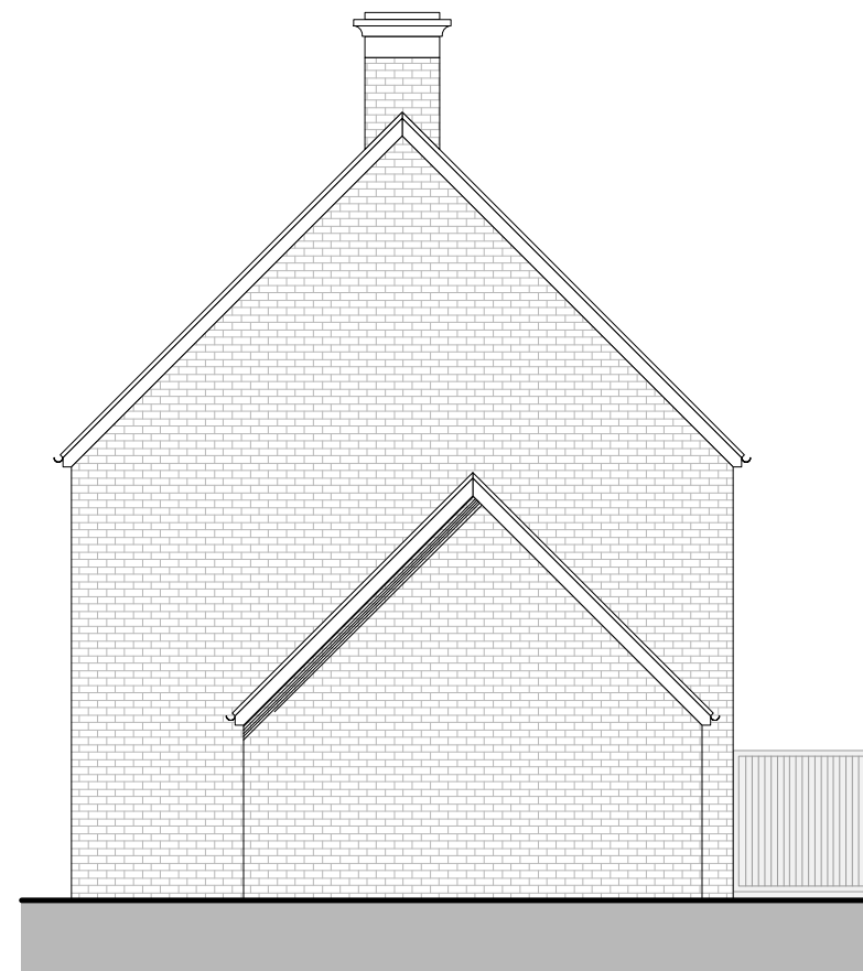
House 89 East elevation
