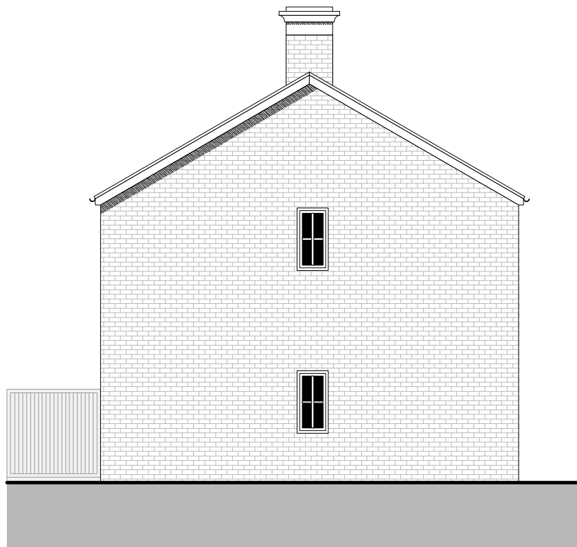
House 53 North elevation
