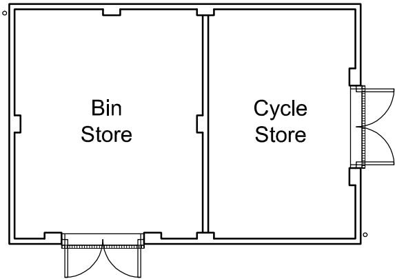
Bin & Bicycle store plan
