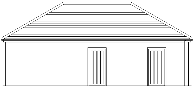
North elevation - Garages 38, 39 & 40
