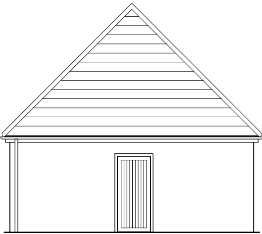
East elevation - Garages 36 - 41
