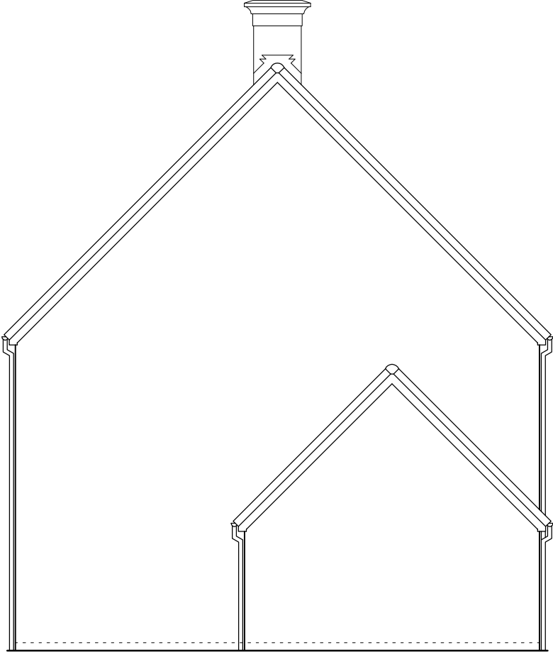
North elevation - Houses 86
