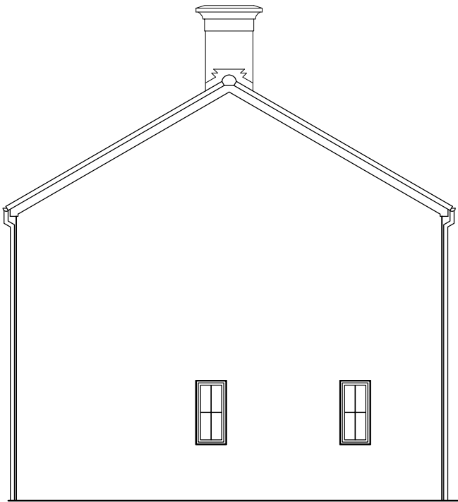
South elevation
