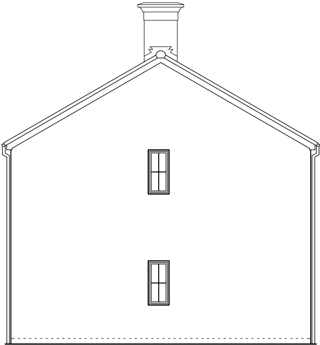
House 55 South elevation
