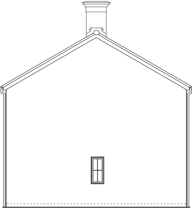
House 53 North elevation
