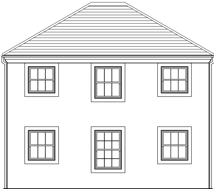
House 51 & 52 South elevation
