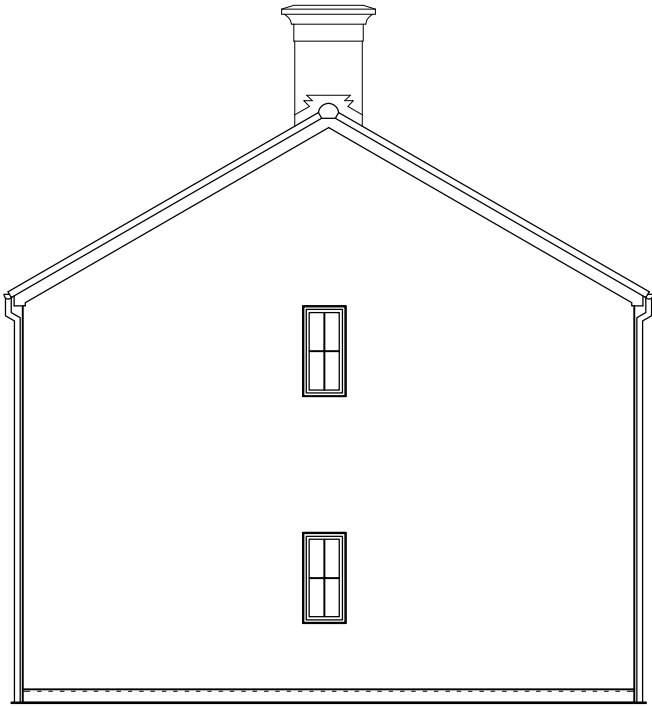
House 42 South elevation
