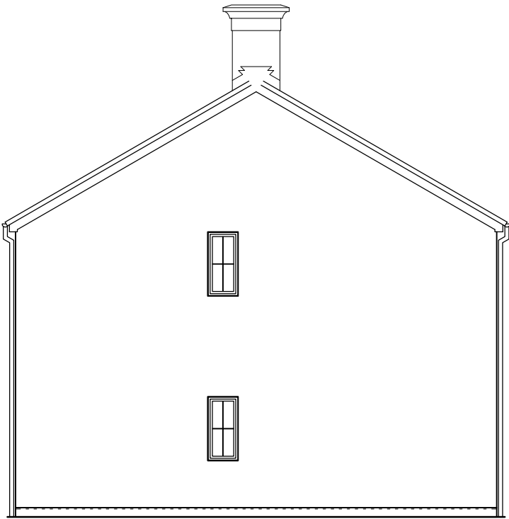
House 27 East elevation
