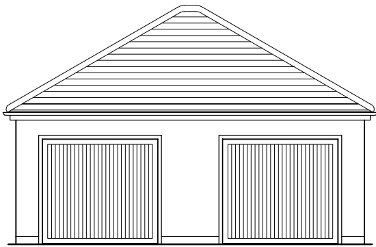
South elevation - Garages 73 - 29
