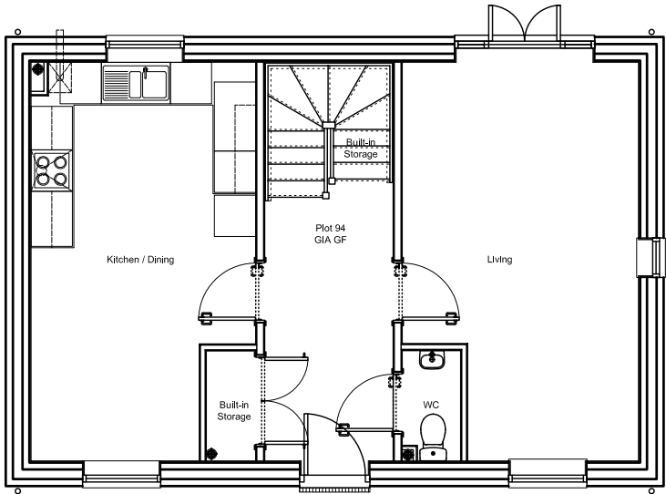
House 94
