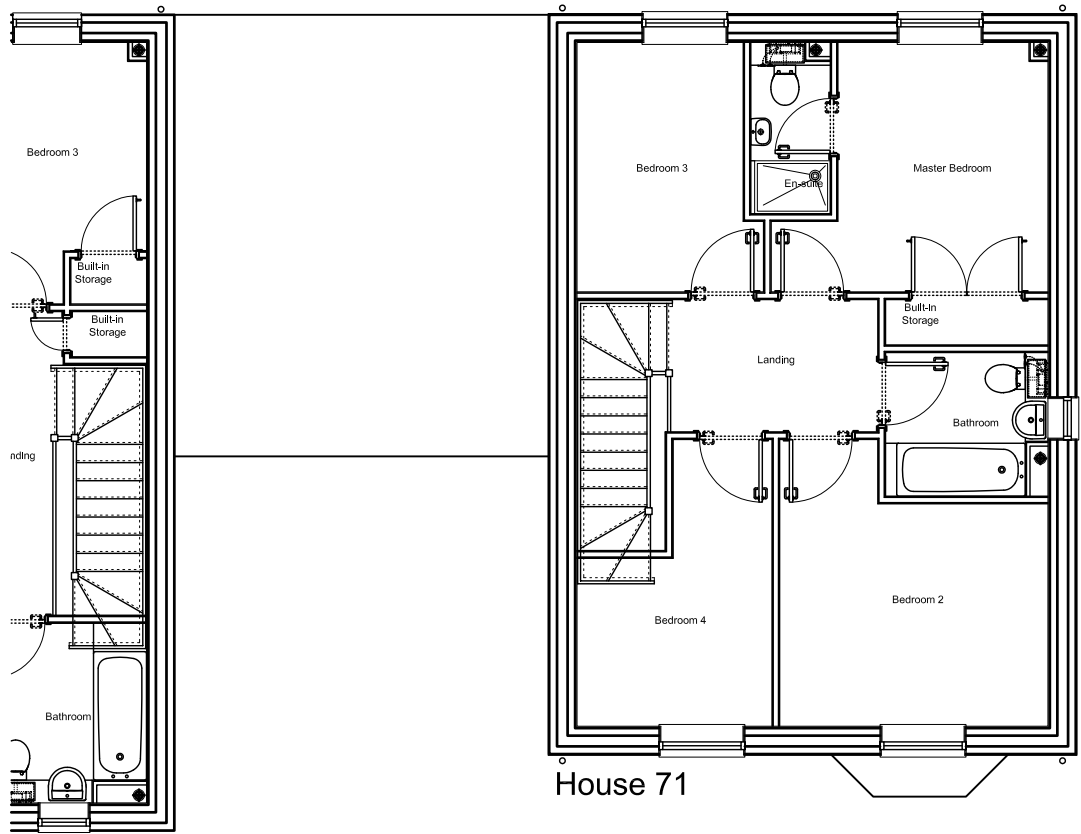
First floor plans
