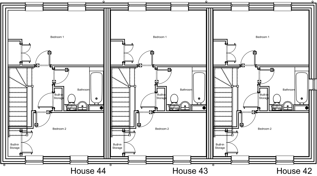
First floor plans
