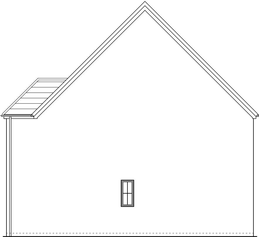
House 40 West elevation
