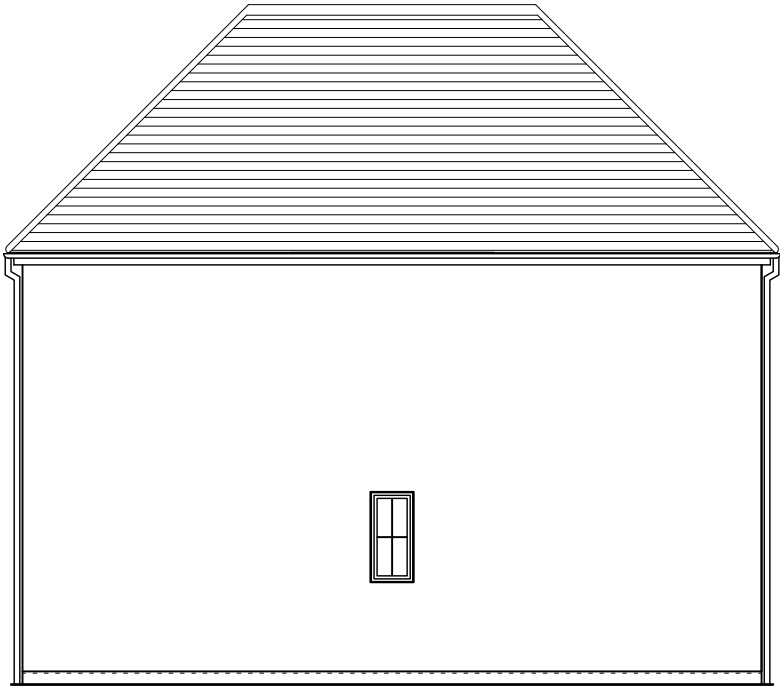
House 33 East elevation
