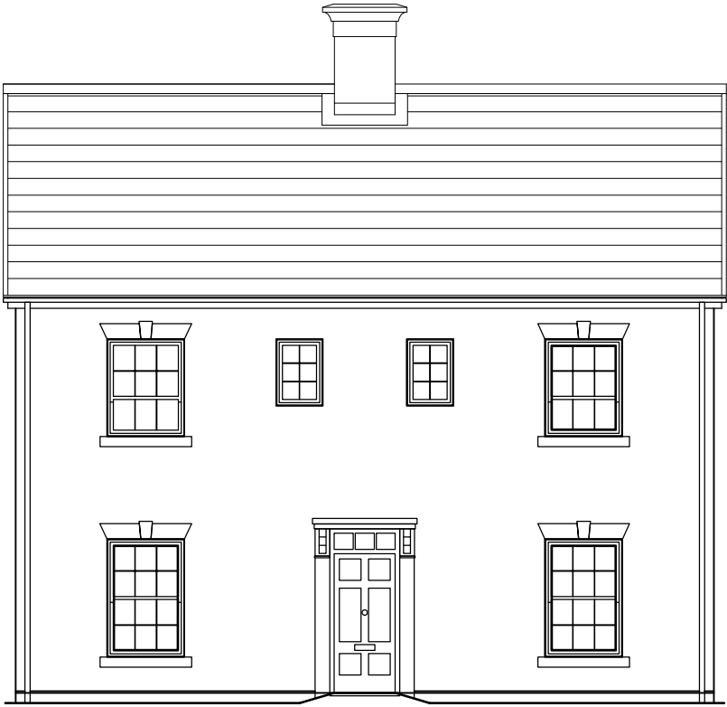
West elevation
