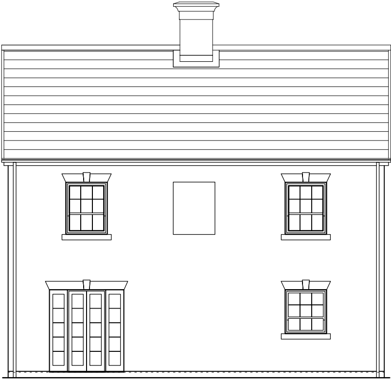
East elevation
