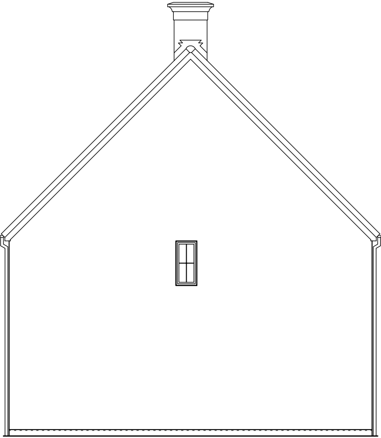
House 24 East elevation
