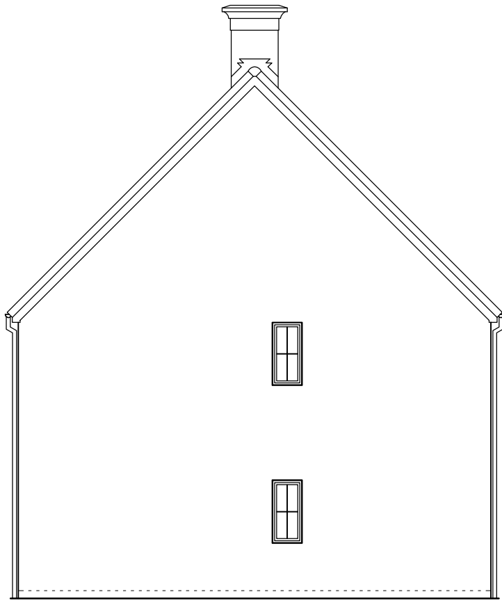
House 18 South west elevation
