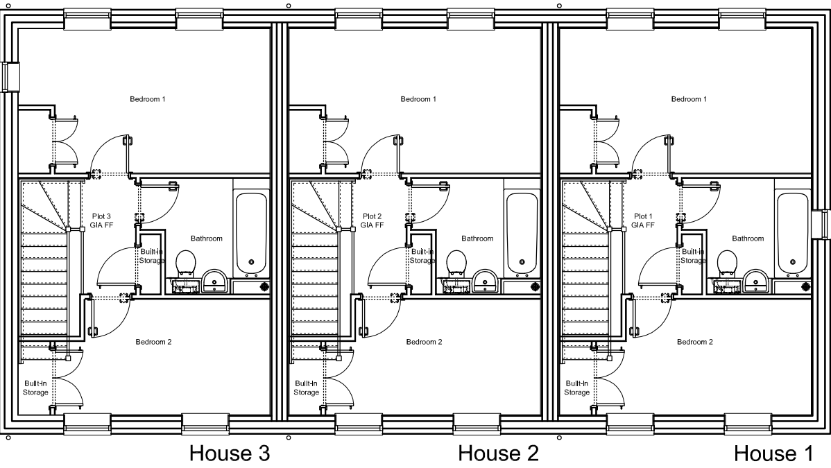
First floor plans
