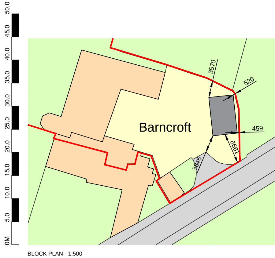
BLOCK PLAN - 1:500
