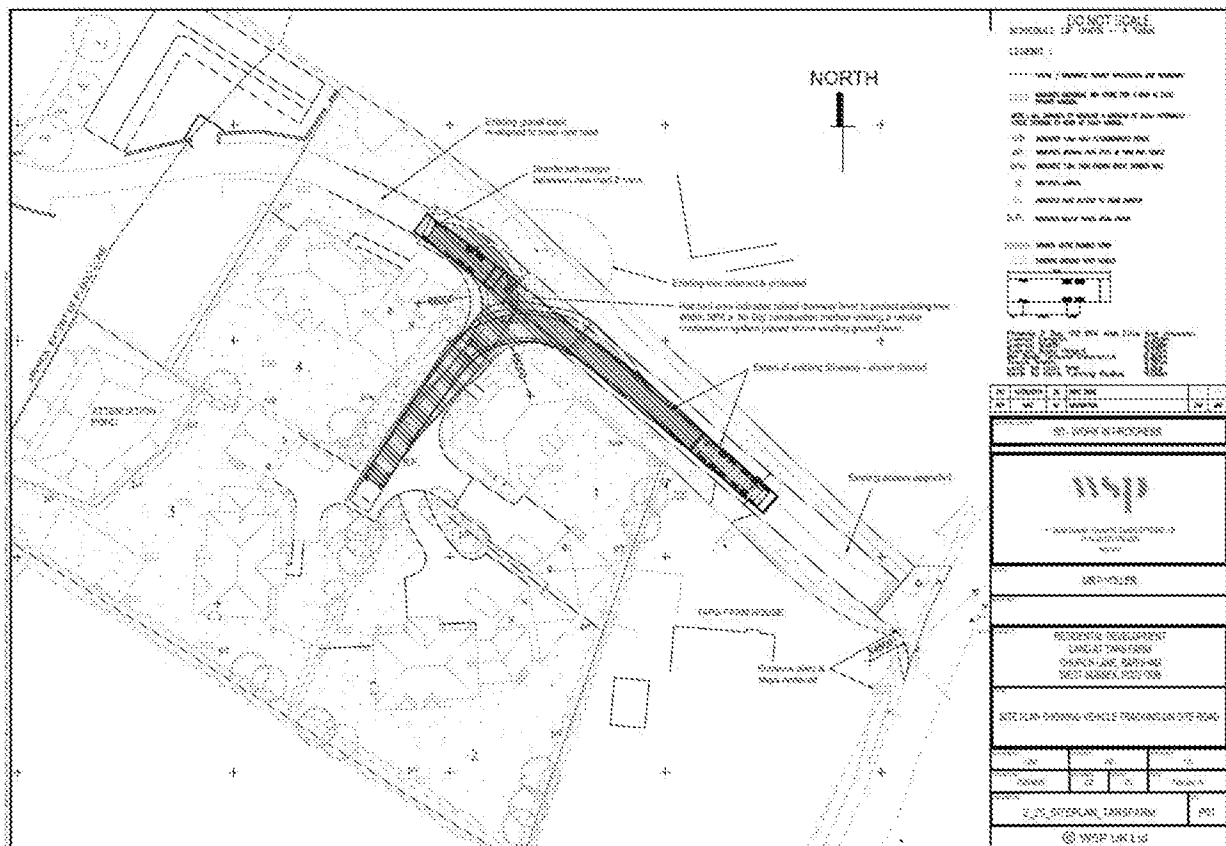
Figure 7: Swept Path Assessment
