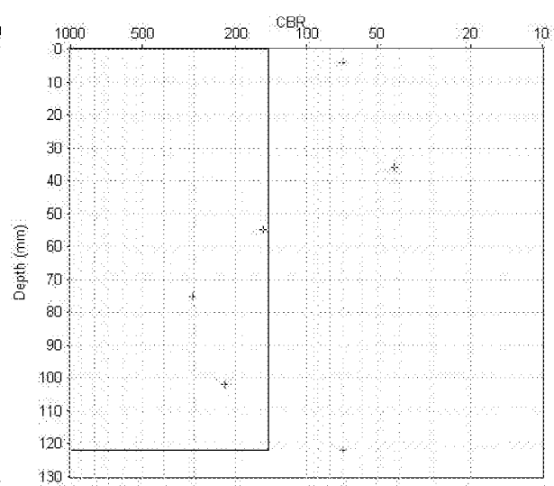
CBR Chart
