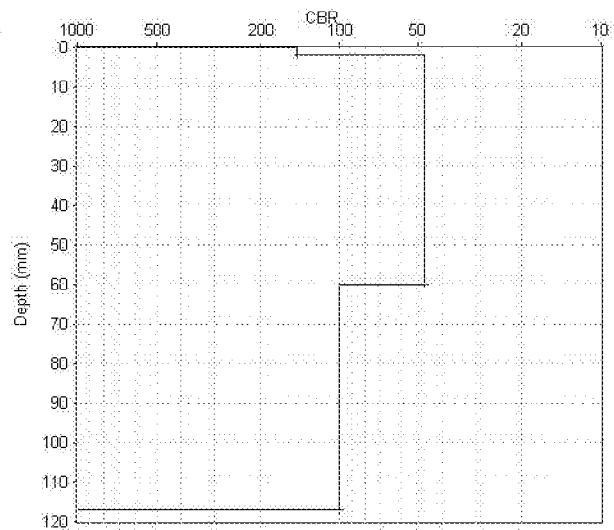
CBR Chart
