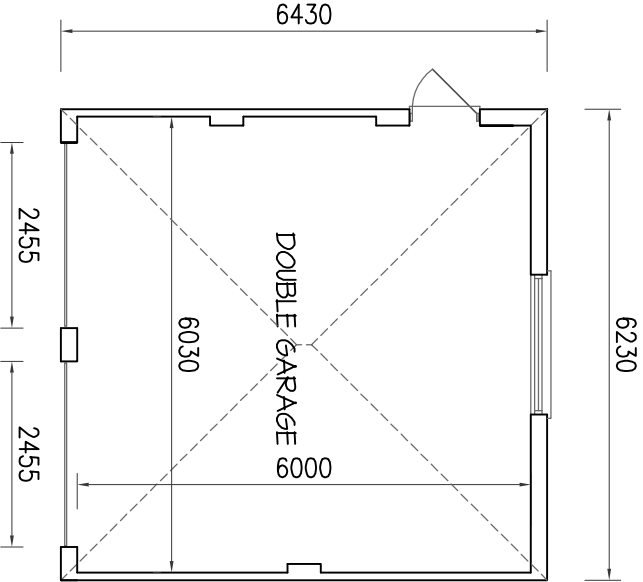
GARAGE FLOOR PLAN
