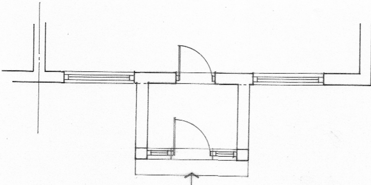
plan of proposed porch 1:50
