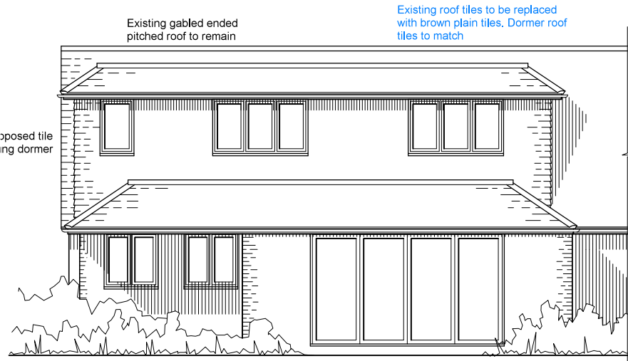
North Elevation
