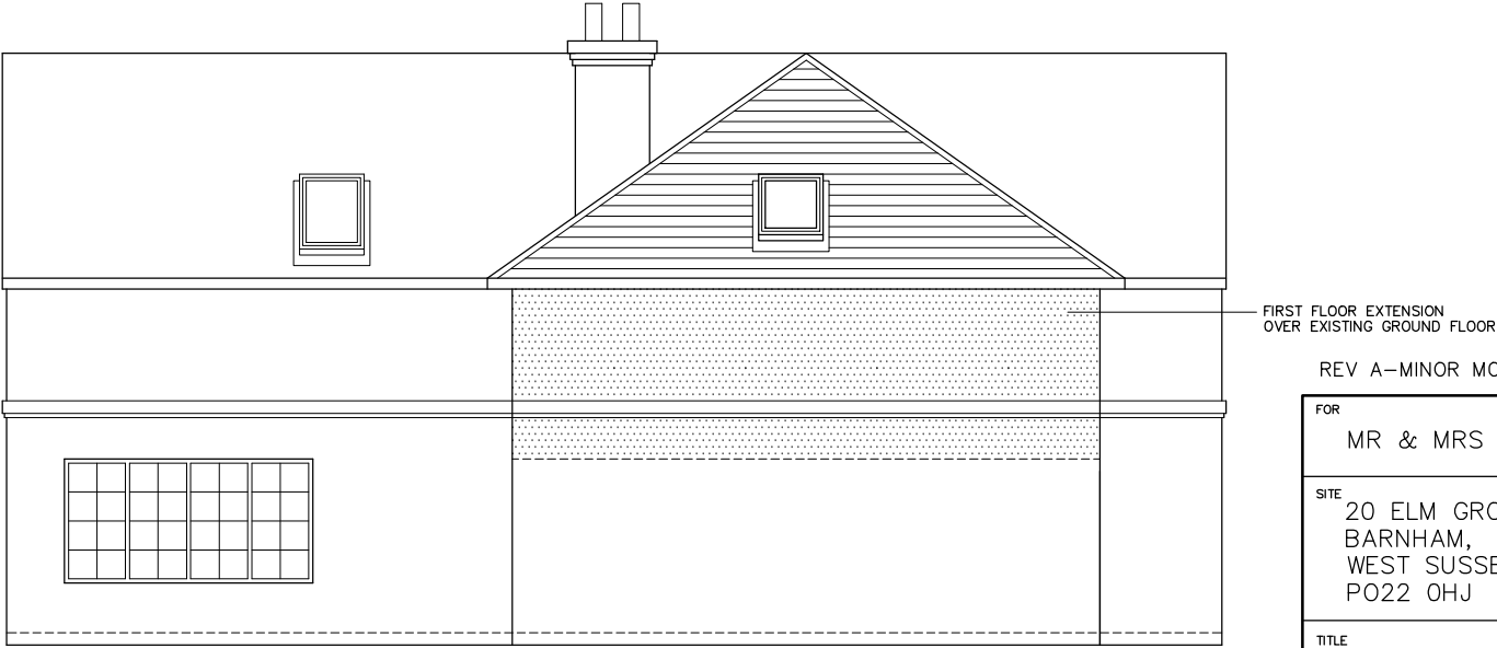
SIDE – NORTH–WEST
