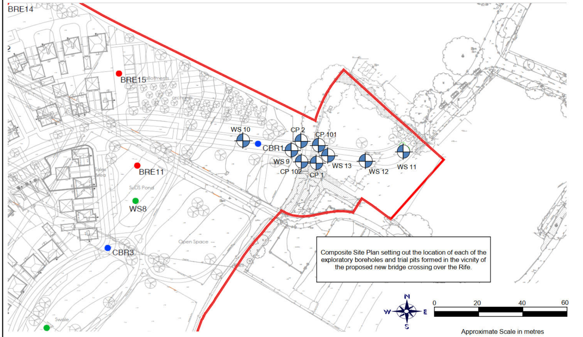
Site Plan - Bridge Area
