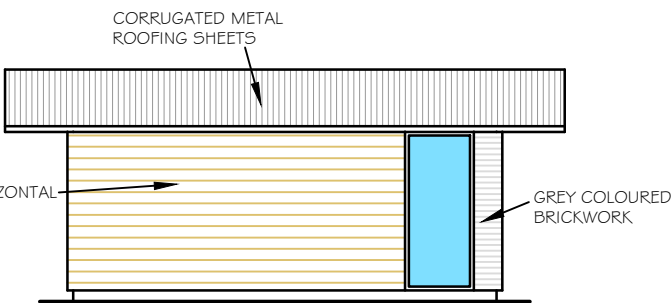
WEST ELEVATION
